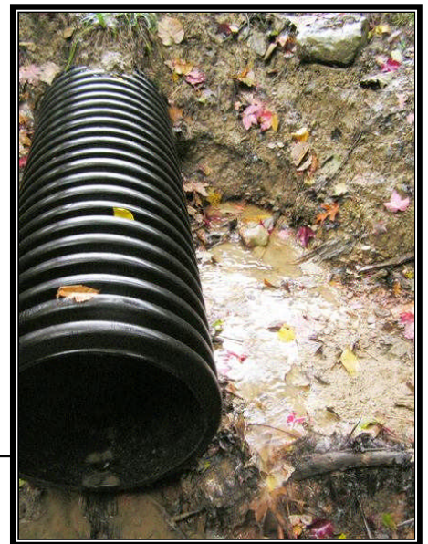
(Above) Water "piping" on the outside of a corrugated pipe following the annular space in the trench (preventable with an anti-seep plug of AquaBlok)
