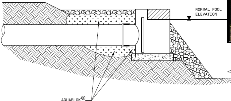
(Above) Water "piping" on the outside of a corrugated pipe following the annular space in the trench (preventable with an anti-seep plug of AquaBlok)
