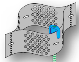
Figure 3 ATRA® Stake Clip
